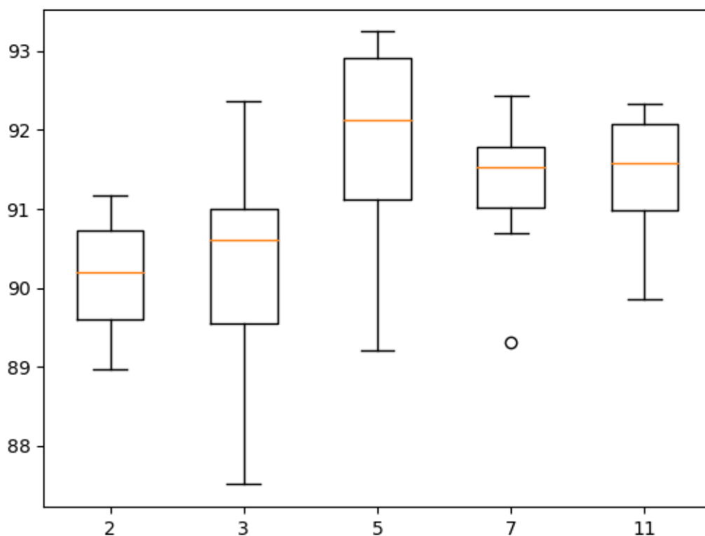
Figure 24.4: Box and whisker plot of 1D CNN with different numbers of kernel sizes.
